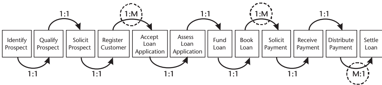
Figure 3.10 Analyzing relationships between processes.
