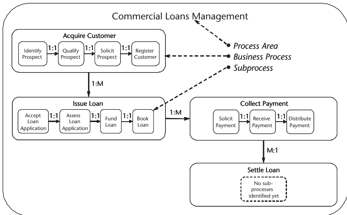
Figure 3.12 Process area, business processes, and subprocesses.
